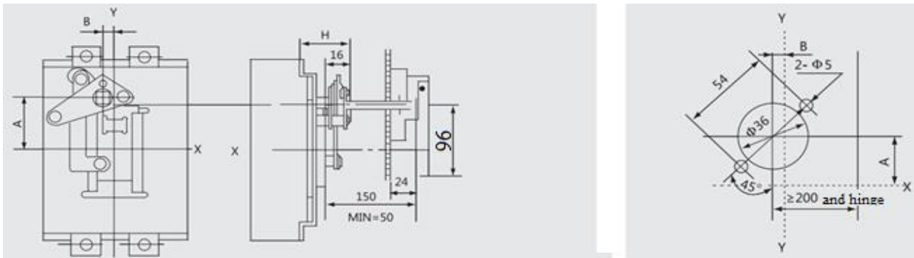
7.2.4 Manual operating mechanism and CS2-F handle
