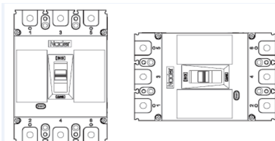
Vertical Installation
