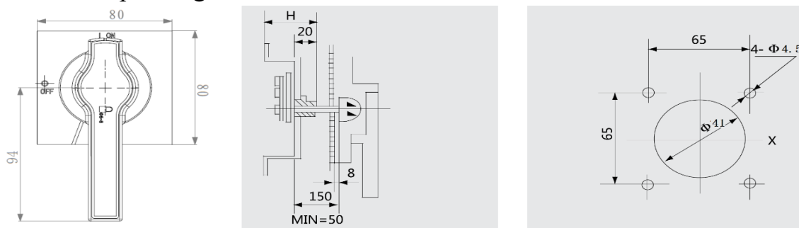
7.2.6 Manual operating mechanism and CS2-IP65 handle
